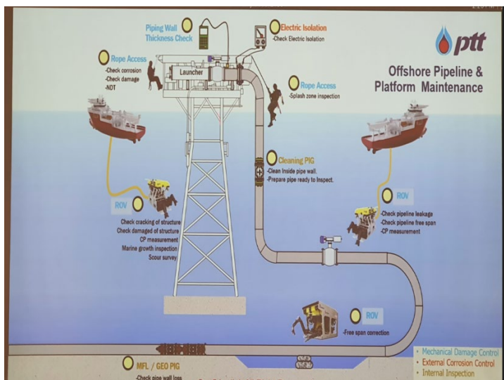
Figure 5: Offshore pipeline maintenance
