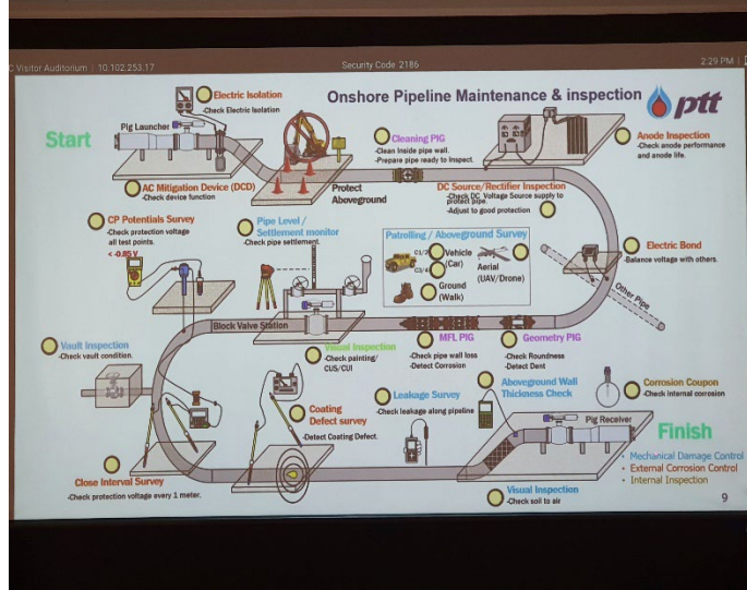
Figure 6: Onshore pipeline maintenance
